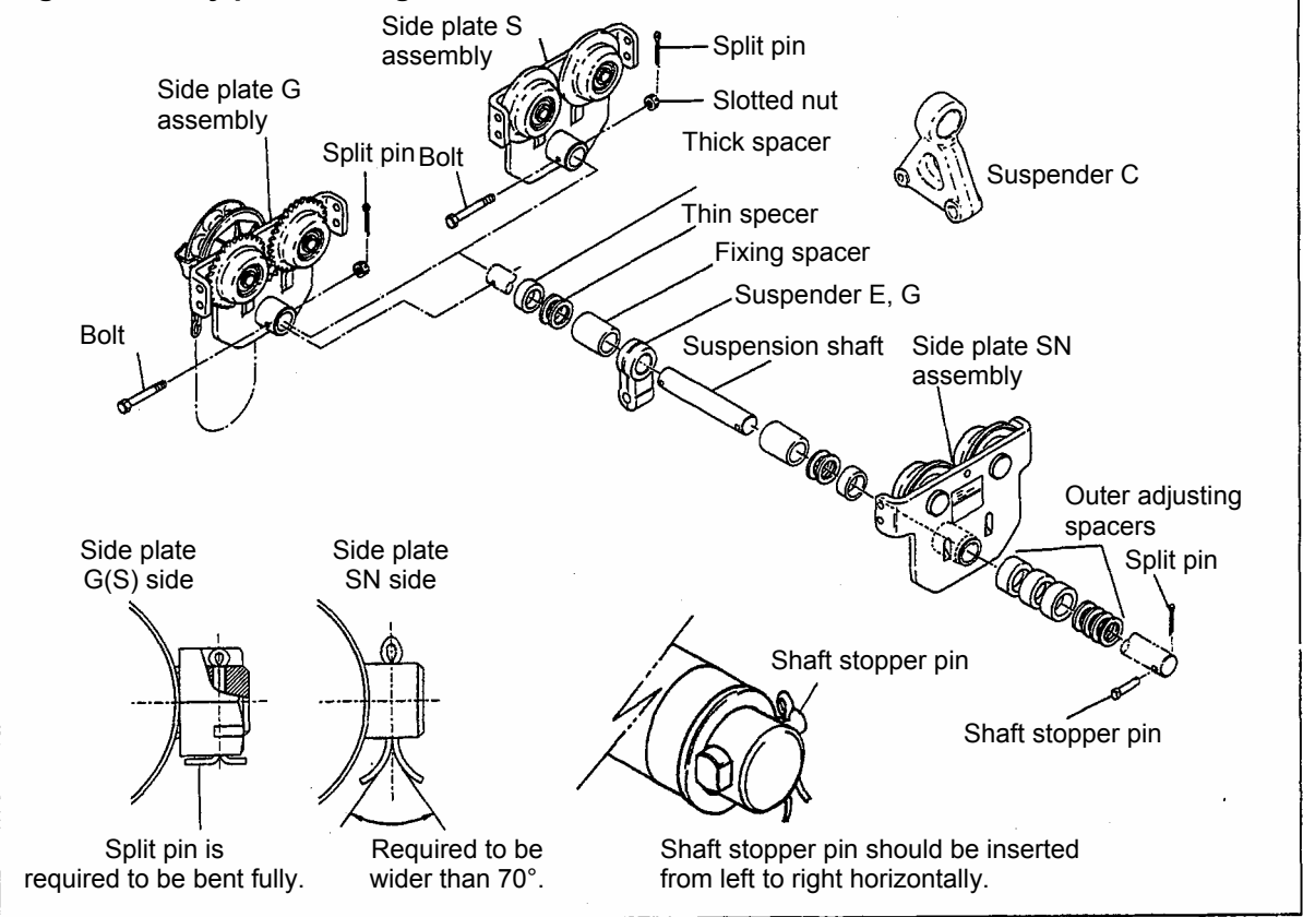
Fig. 8-2 Trolley parts arrangement - for 5t
