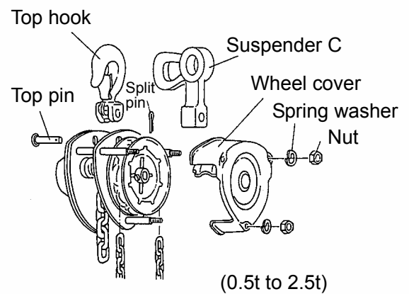
Fig. 5-4 Mounting suspender C
