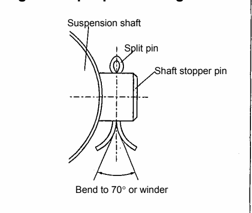
Fig. 5-12 Split pin bending
