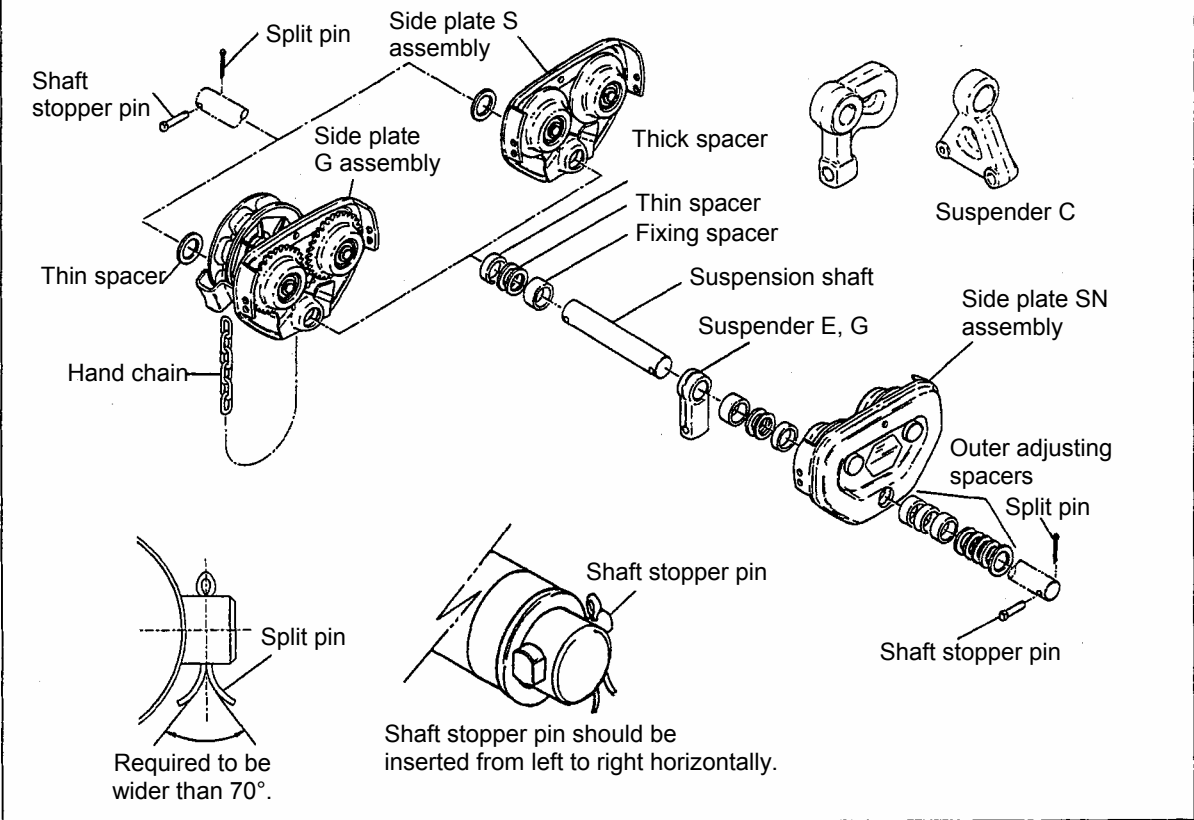
Fig. 8-1 Trolley parts arrangement - for 3t and smaller
